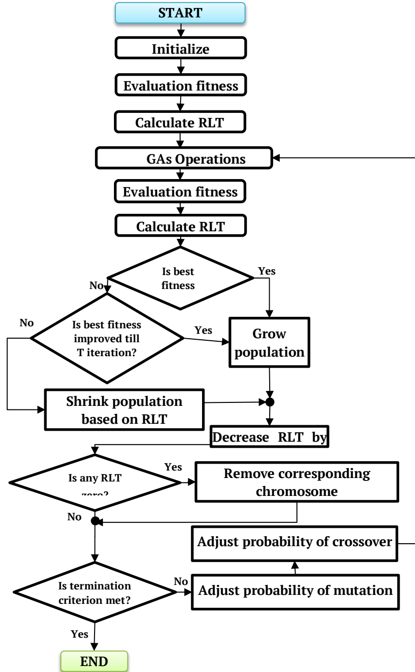
Figure 2: Flowchart of APGA. Adapted from [9].
