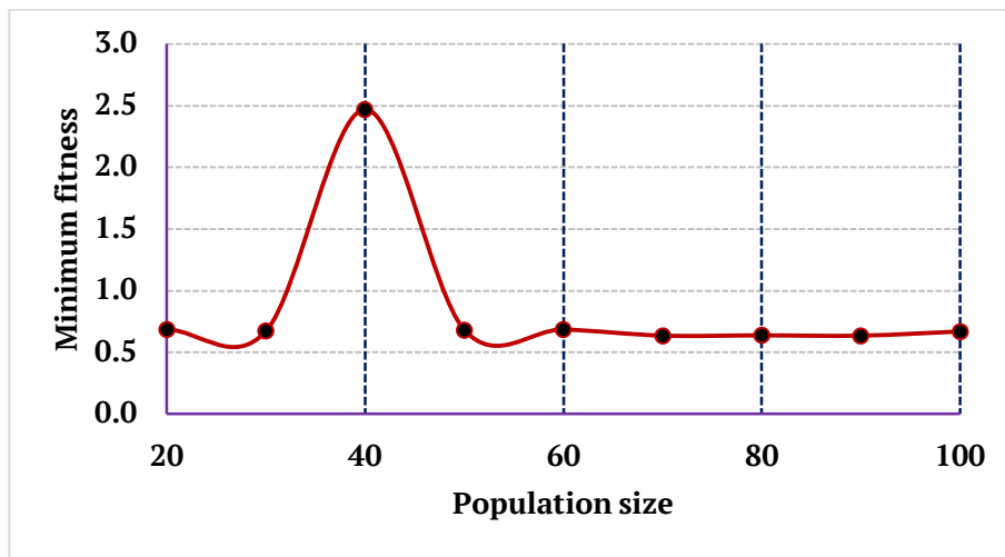
Figure 3: Sensitivity analysis for the population size of AGA model
