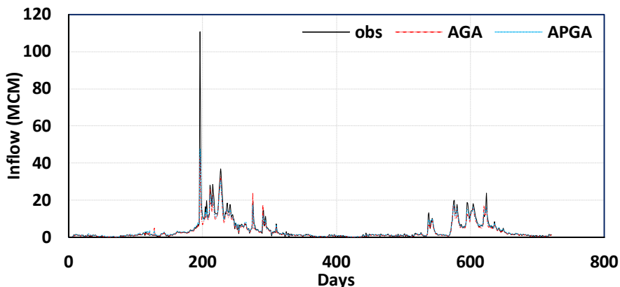
Figure 9: The comparison of inflow from observation data, APGA, and AGA models during the testing period.
