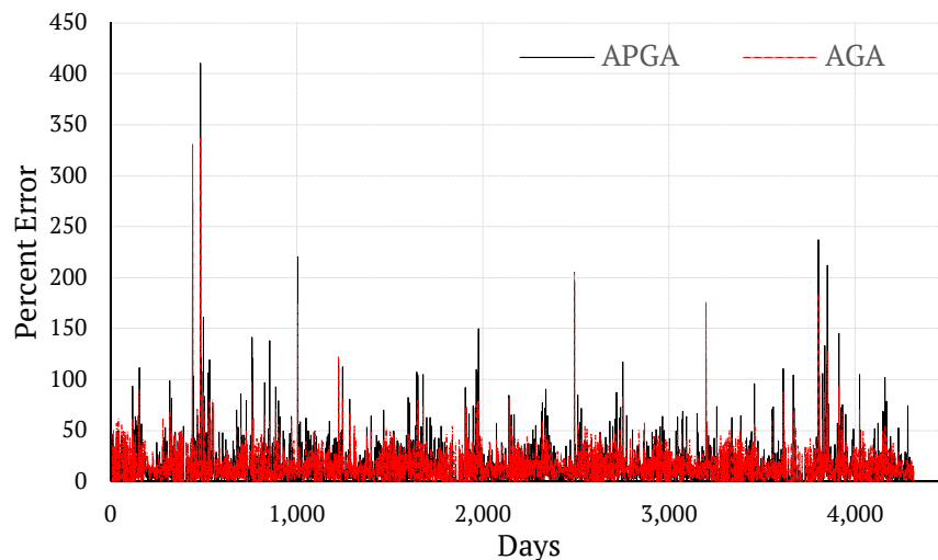
Figure 5: The comparison of percent error from APGA and AGA models during the training period
