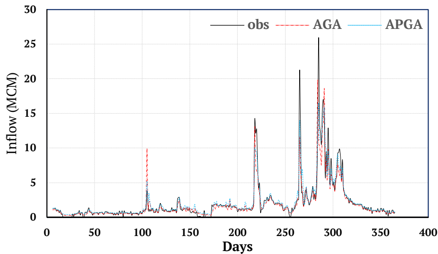
Figure 10: The comparison of inflow from observation data, APGA, and AGA models during the application period
