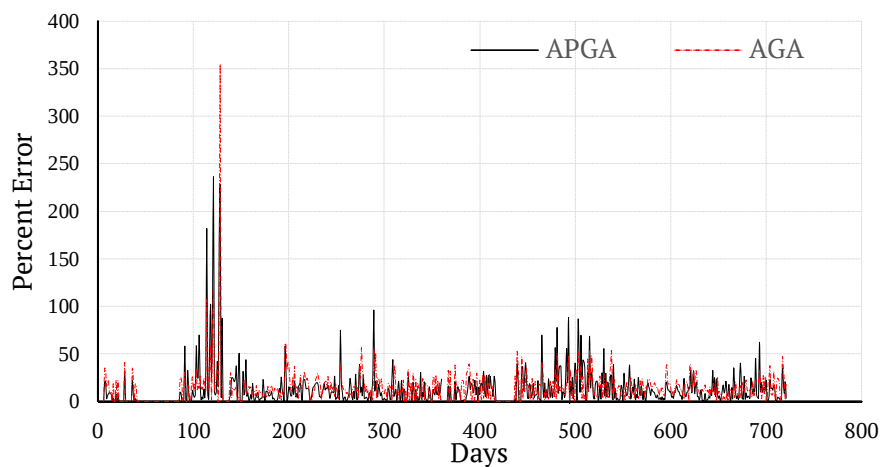
Figure 6: The comparison of percent error from APGA and AGA models during the testing period.
