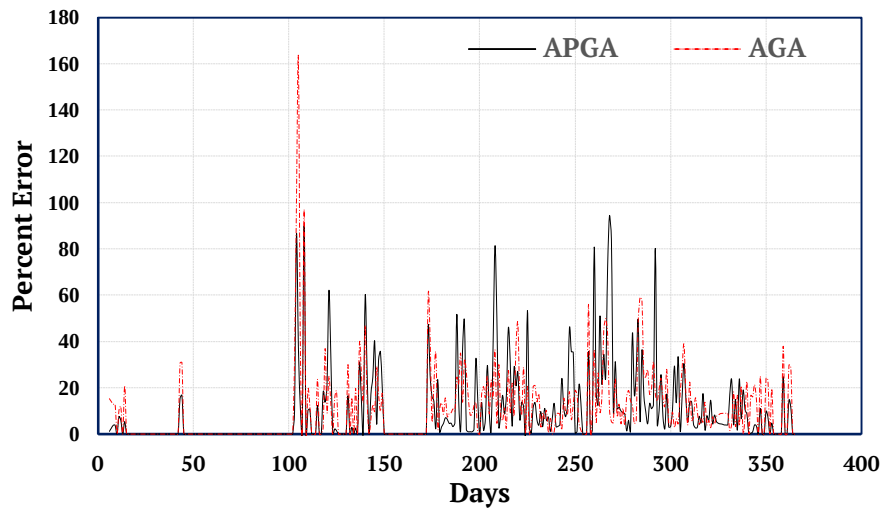
Figure 7: The comparison of percent error from APGA and AGA models during the application period
