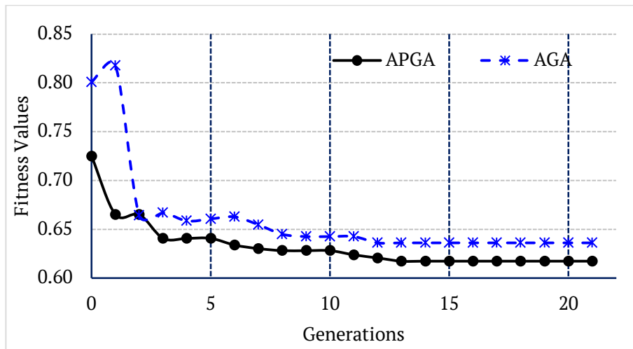
Figure 4: Comparison of the fitness values of the APGA and AGA models.
