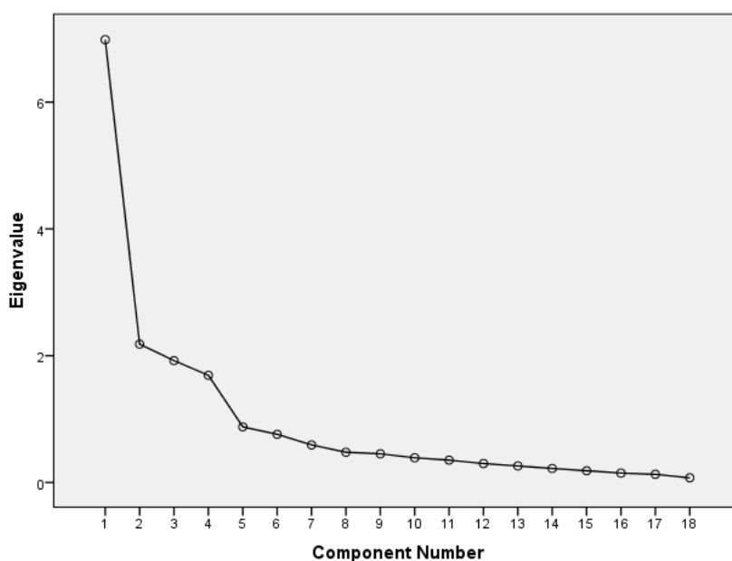
Figure 2: Scree Plot
