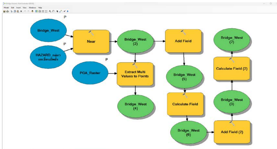
Figure 4: Complete Model Data Flow Diagram
